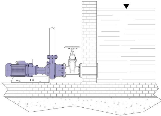
Installation scheme
